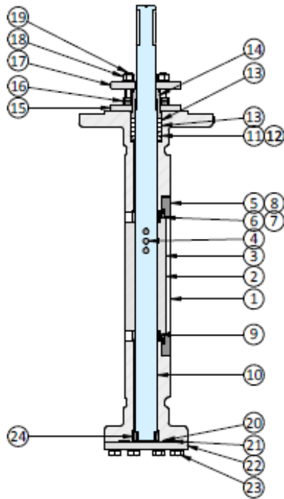
Figure 1: Severn 8500 Series Control Valve – Cut section view.
