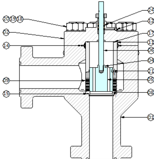
Figure 1: Severn 5200 Series Choke Valve – Cut section view.
