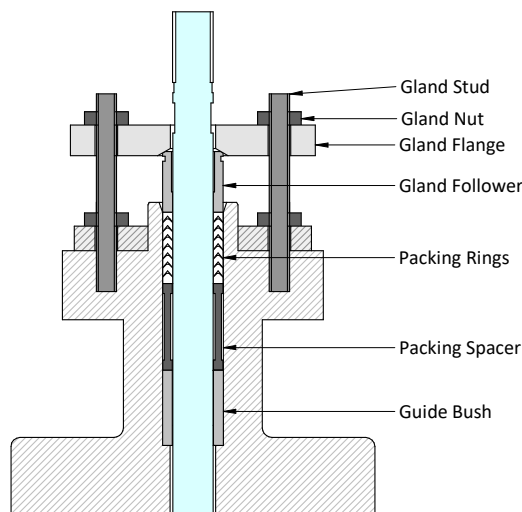
Figure 2: Stuffing Box & Gland Flange Components
