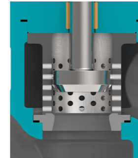
Unbalanced trim
