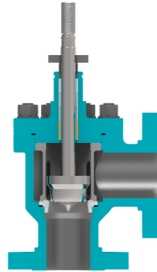
Angle body
