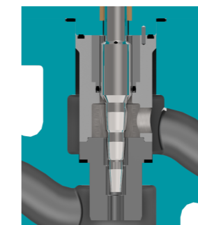
Balanced trim
